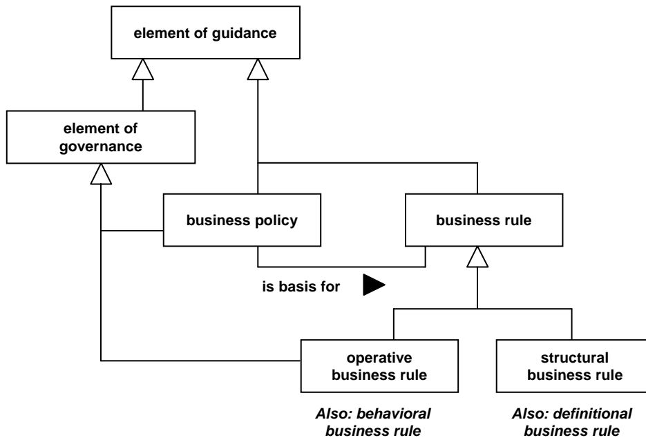
Figure F.4 - Business Rule fragment of SBVR
